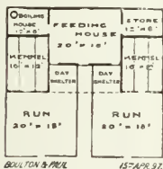
BOULTON AND PAUL'S HOUND KENNELS.
